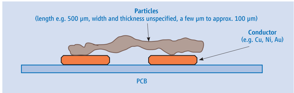
Fig. 88: Sketch of electrical arrangement (particle forming “bridge” between two conductors)
