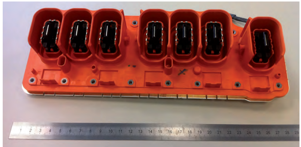
Fig. 13: Evaluation of 7-pin HV strip connector
