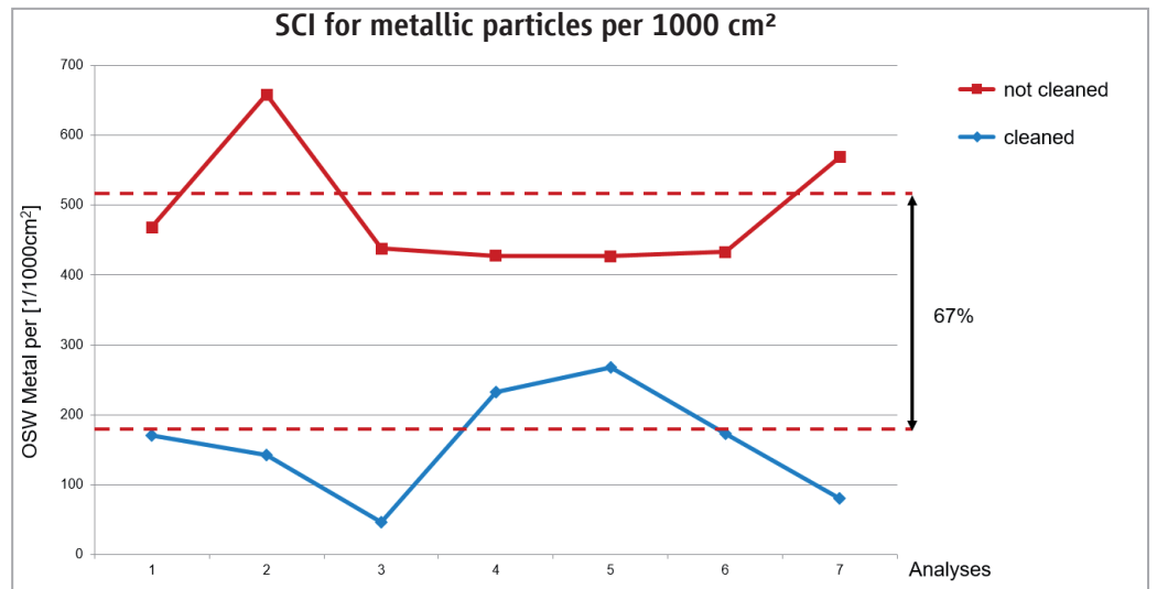
Fig. 14: Graph showing cleaning effect based on SCIs
