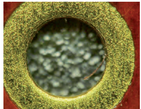
Fig. 63: Chip formation caused by stamping
