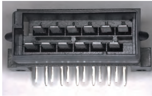
Fig. 52, 53: 12-pin connector with bridged contacts
