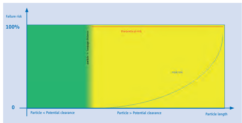
Fig. 87: Diagram showing failure risks based on metallic particles on assemblies
