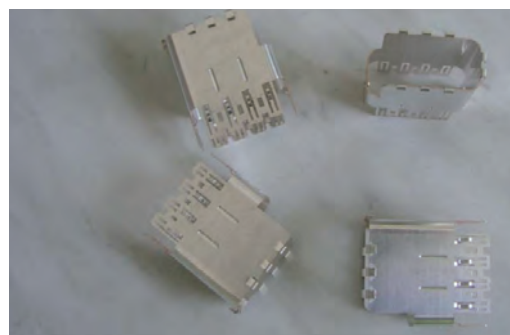
Fig. 36,37,38: Shielding plate
